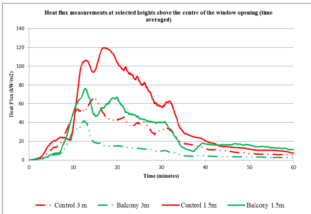
Figure B.4 –Comparison of heat flux measurements at selected heights above the window opening
