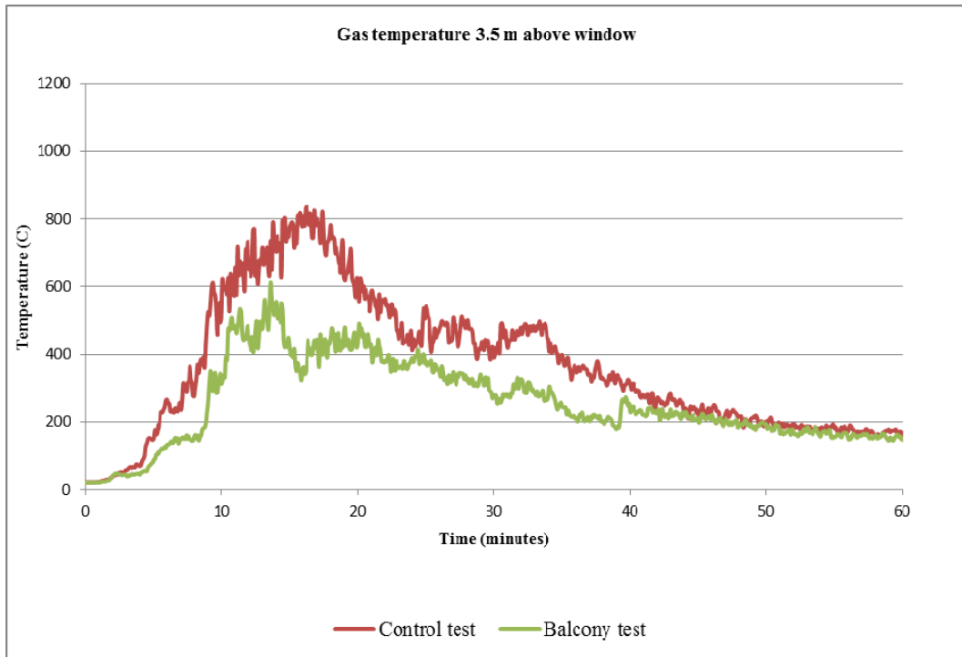
Figure B.11 –Gas temperature at 3.5 m above window opening
